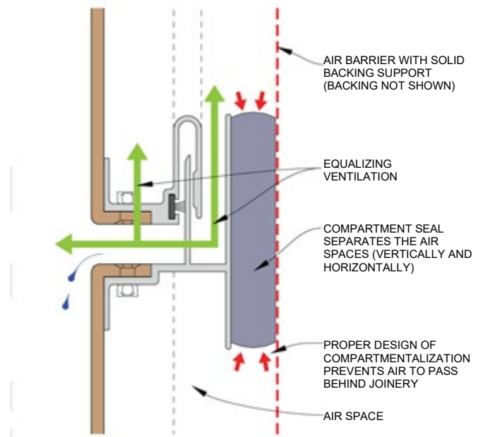
Figure 6 – Pressure Equalized Rainscreen System Horizontal Joint (Example)
